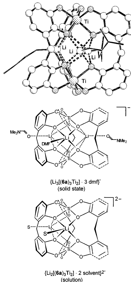
Fig. 5 The molecular structure of Li_3[(\mathbf{6a})_3Ti_2]^- in the solid state and of Li_2[(\mathbf{6a})_3Ti_2]^{2-} in solution
