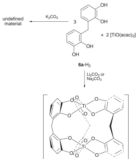
Scheme 2 Template-directed self-assembly of [(\mathbf{6a})_3Ti_2]^{4-}
